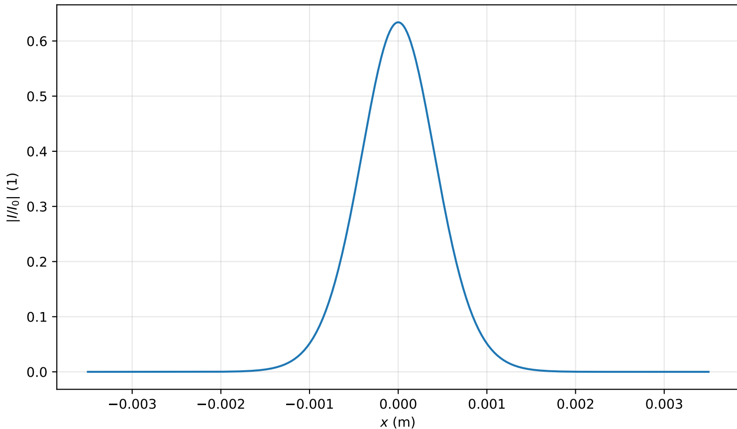
Intensity profile I(x, y = 0, z = 2.070m)/I_0 , P_{in}=0.3P_{cr} , artificial time
